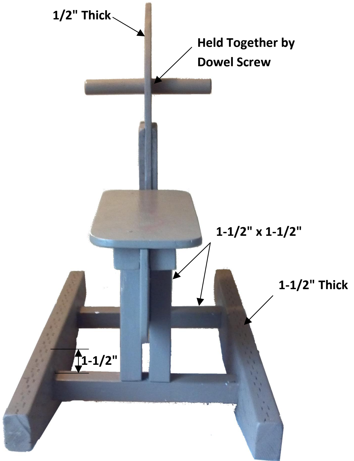
Dowel Screw
